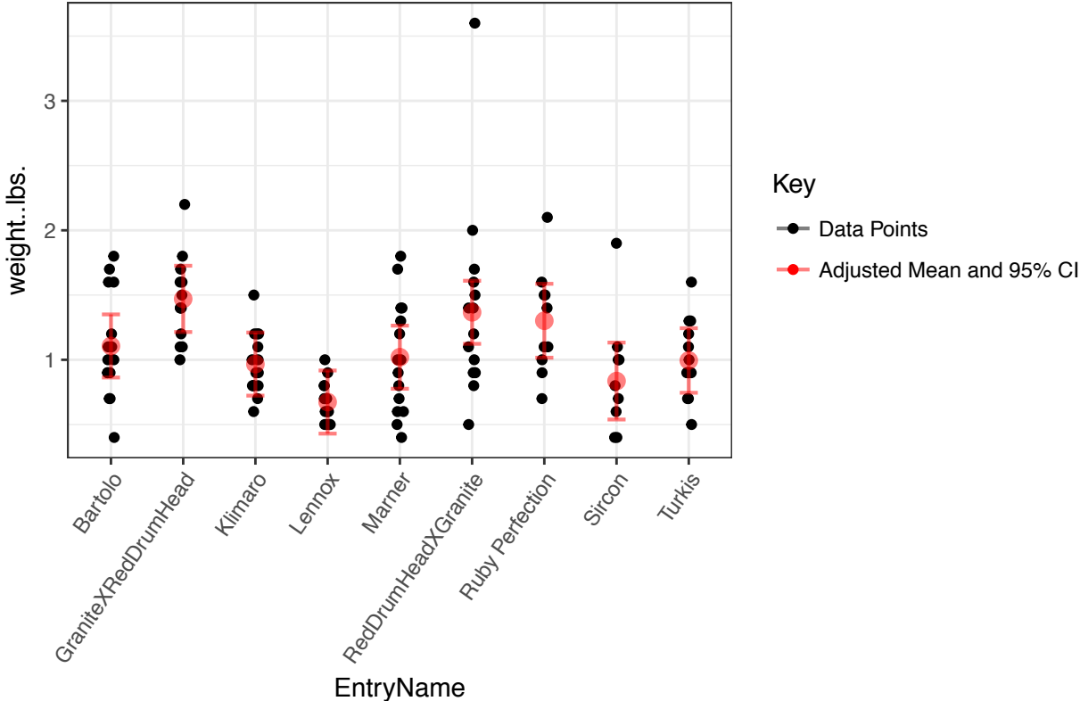
Plot of means and confidence intervals for weight..lbs.
