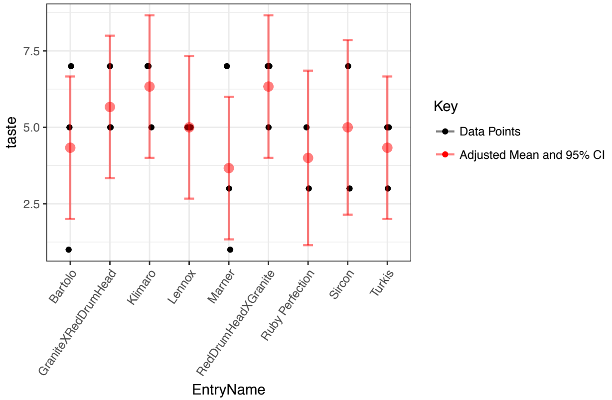
Plot of means and confidence intervals for taste
