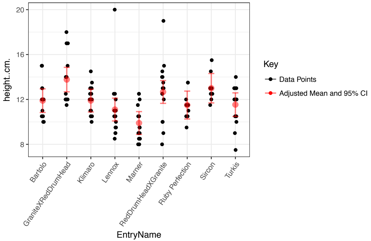
Plot of means and confidence intervals for height..cm.
